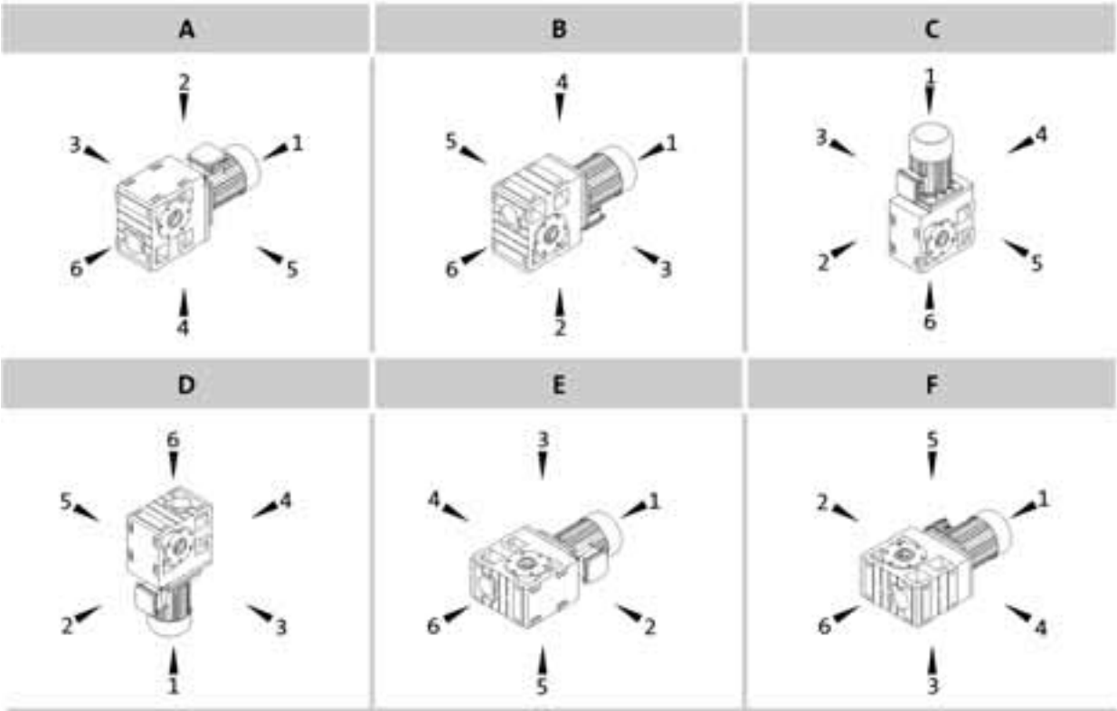
Mounting position (A...F) and position of system blocks (1...6)
